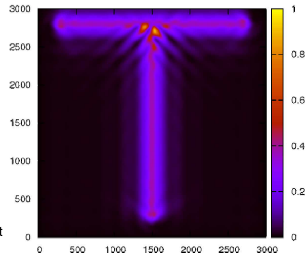
Intensity in resist without and with silver slab
