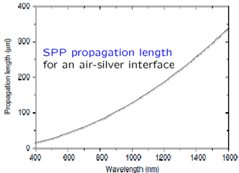
Figure 5. Showing the propagation length of the surface plasmon-polariton. The data were computed using the Drude approximation for the relative permittivity for the metal (with \omega_p and \Gamma for silver taken to be \omega_p = 1.2 \times 10^{16} \text{ rad s}^{-1} ( \approx 7.9 \text{ eV} ) and \Gamma = 1.45 \times 10^{13} \text{ s}^{-1} ( \approx 0.06 \text{ eV} ) respectively). The relative permittivity of the dielectric was taken to be equal to 1. Note that in calculating these data we have assumed that there is no radiative damping, specifically that there is no mechanism by which SPPs can be converted to light, e.g. by the presence of a prism or grating coupler.
