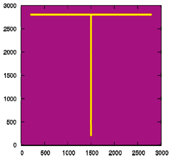
Chromium mask with 40 nm wide PMMA slots ( \epsilon_r = 2.4 )
