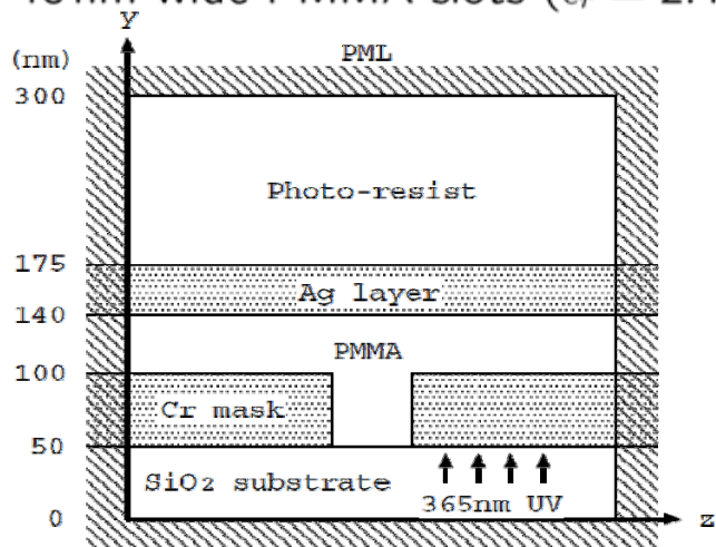
Chromium mask with 40 nm wide PMMA slots ( \epsilon_r = 2.4 )
