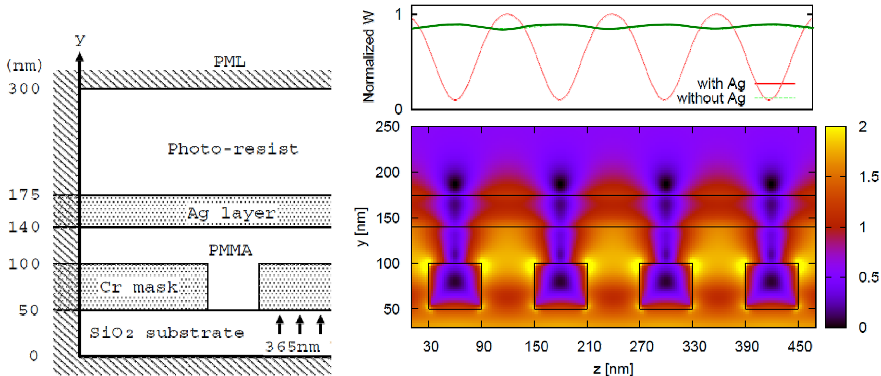
Fig. 4. Imaging of a grating (60 nm wide slit and 60 nm wide Cr mask). Top: a linear scale profile of the grating image obtained by integrating the energy dissipation W in the photo-resist layer observed at height 180 nm. The image profile for the case of no silver layer is plotted for comparison. Bottom: the distribution of W on the cross section in a logarithmic magnitude color scale. The black solid lines indicate the boundaries of the Ag film (140 nm to 175 nm in height) and Cr mask of the grating (50 nm to 100 nm in height).
